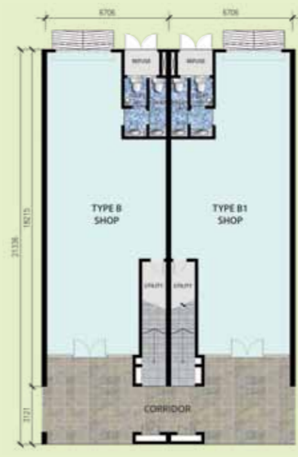
TYPE B & B1 GROUND FLOOR
